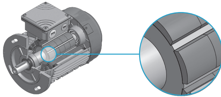
SMPM Design Surface Mounted Permanent Magnets
