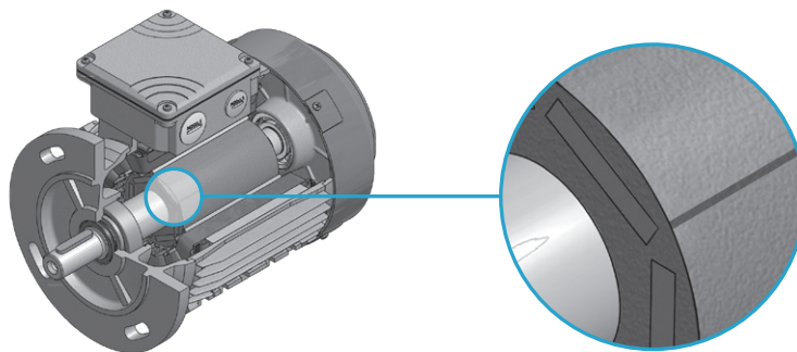
IPM Design Interior Permanent Magnets
